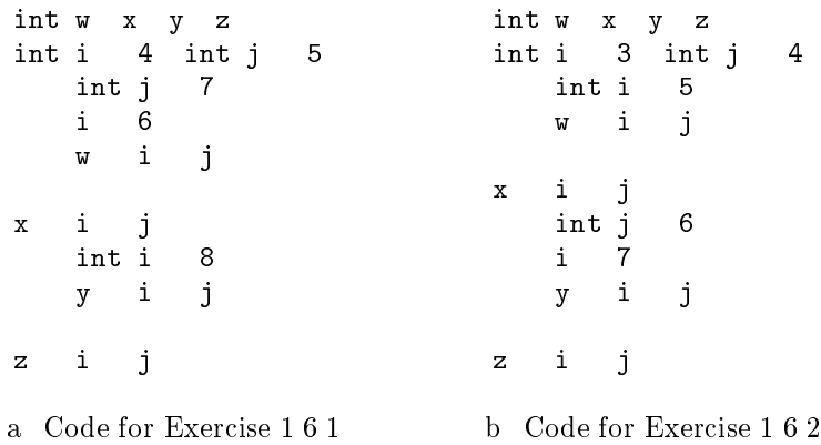
Figure 1 13 Block structured code
