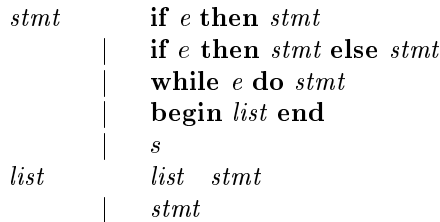
Figure 4 56 A grammar for certain kinds of statements
