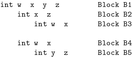
Figure 1 13 Block structured code
