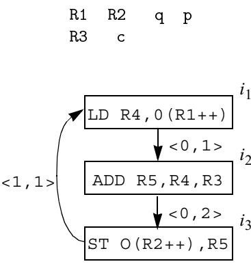
Figure 10.25 Data dependence graph for Example 10.18
