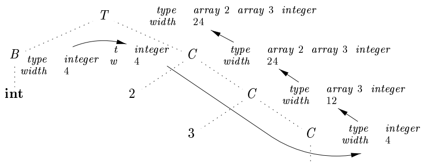
Figure 6 16 Syntax directed translation of array types
