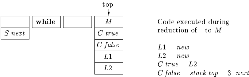
Figure 5.36 LR parsing stack after reduction of \rightarrow M
