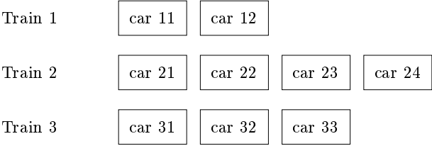
Figure 7.30 Organization of the heap for the train algorithm
