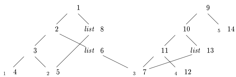
Figure 6 33 Initial graph with each node in its own equivalence class
