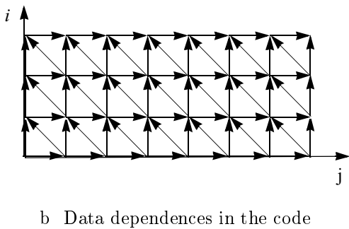
Figure 11.50 An example of successive over relaxation (SOR)
