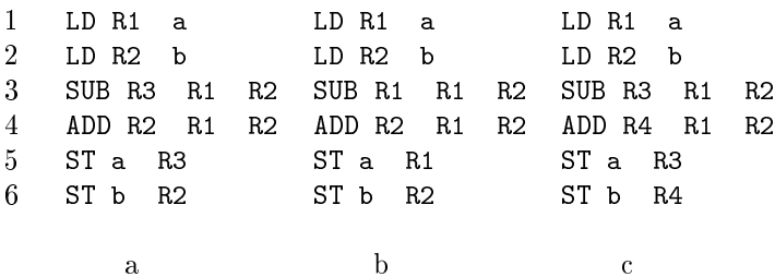
Figure 10 10 Machine code for Exercise 10 3 1
