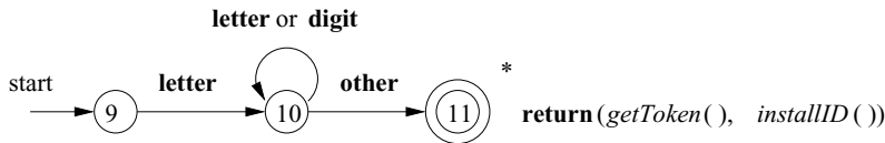
Figure 3.14 A transition diagram for identifiers and keywords
