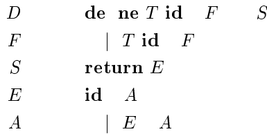
Figure 6 52 Adding functions to the source language
