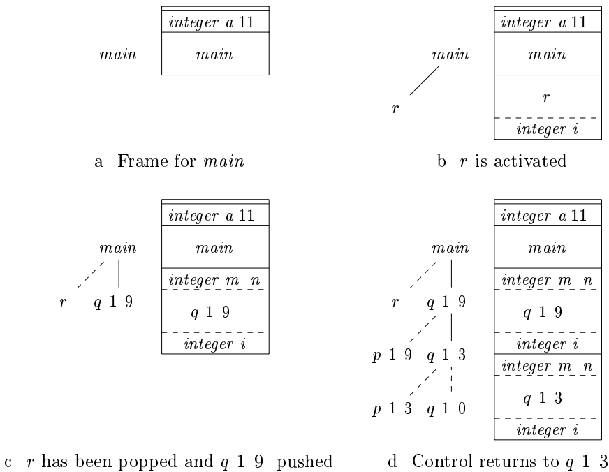
Figure 7.6 Downward growing stack of activation records
