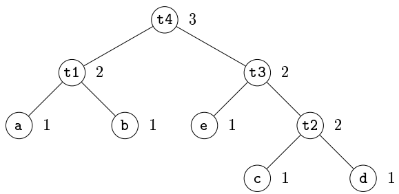
Figure 8 23 A tree labeled with Ershov numbers
