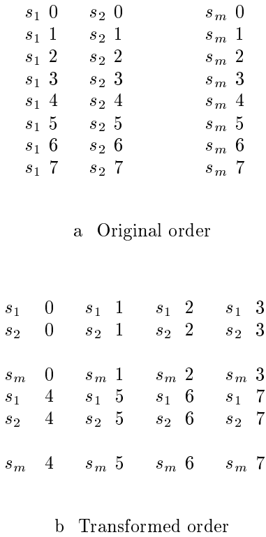
Figure 11 65 Distributing a stripmined loop
