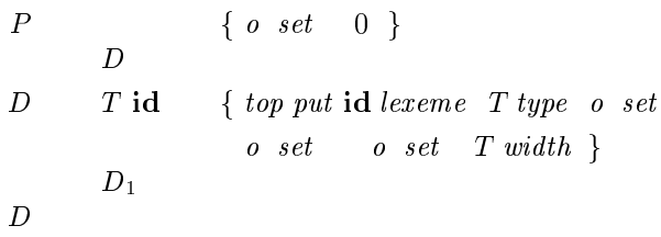
Figure 6.17 Computing the relative addresses of declared names
