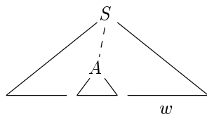
Figure 4.27 A handle A in the parse tree for w
