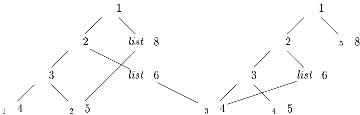
Figure 6 31 Equivalence classes after uni cation
